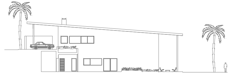
Alzado Sur/South Elevation
